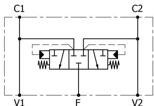
Hydraulic circuit
